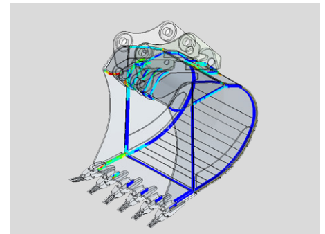
Strength assessment of seam welds on solid structures in ANSYS Workbench with WB/FKM-Weld
