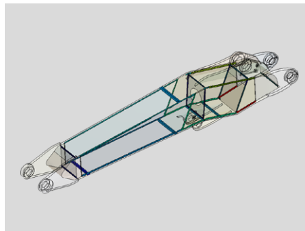
Strength assessment of seam welds on shell structures in ANSYS Workbench with WB/FKM-Weld
